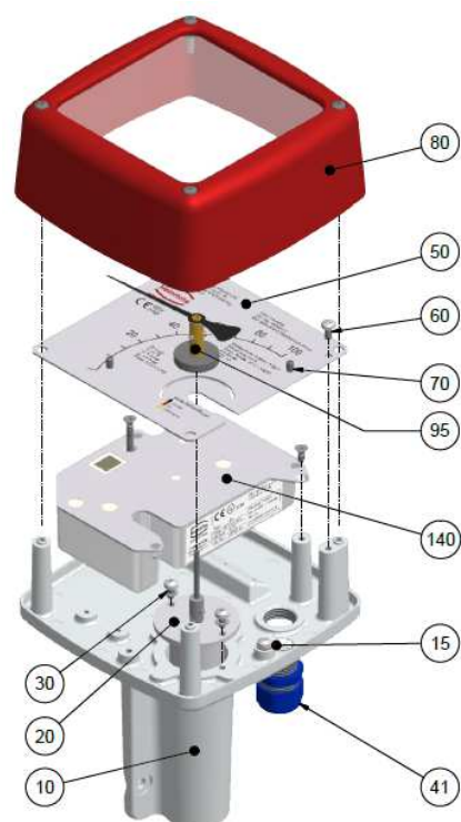
22.2.6 Complete Indicator unit with transmitter ES Ex HART®
